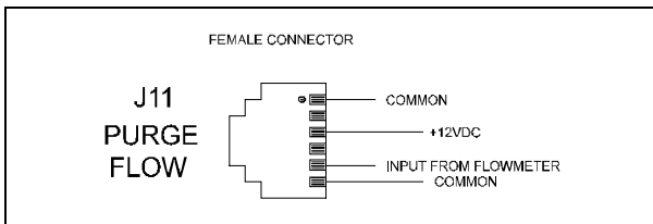
J11 connectors
