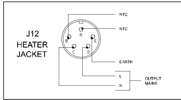
J12 connectors
