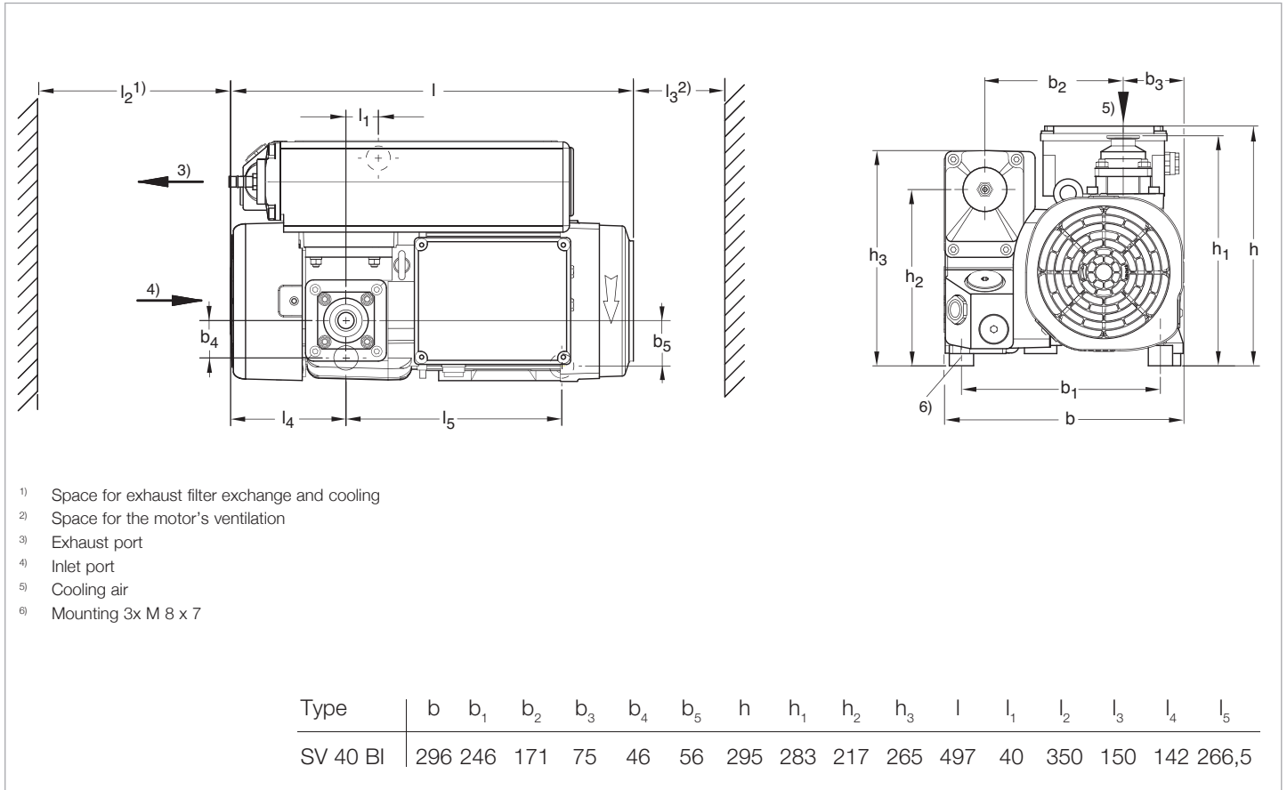
Dimensional drawing for the SOGEVAC SV 40 BI with standard single-phase motor, European version (dimensions for three-phase motor smaller)
