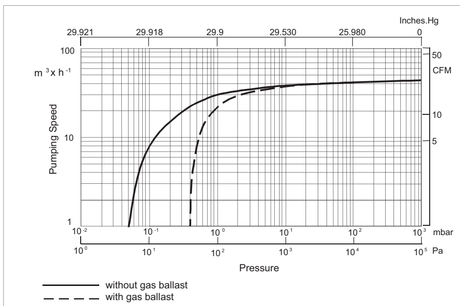
Pumping speed characteristics of the SOGEVAC SV 40 BI at 50 Hz
