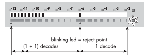
Control panel (plate removed).
