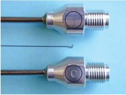
Sniffer probe equipped with a dia. 0.30 mm needle has no mark or is marked "0".
