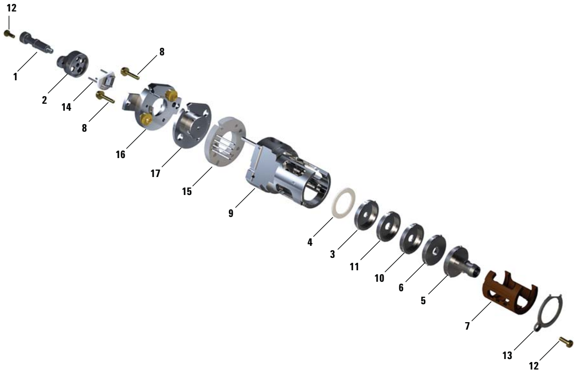
Figure 19 LE-EI ion source
