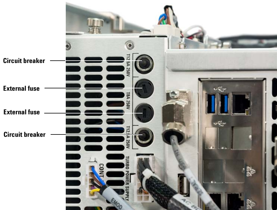
Figure 18 7250 Fuses
