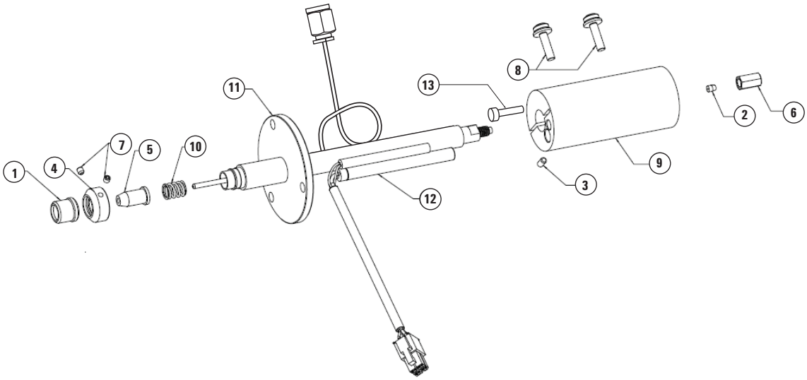
Figure 20 GC/MS Transferline interface for the 7890 GC
