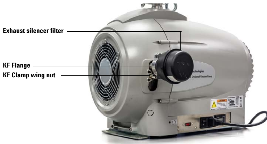
Figure 15 Foreline pump exhaust silencer filter
