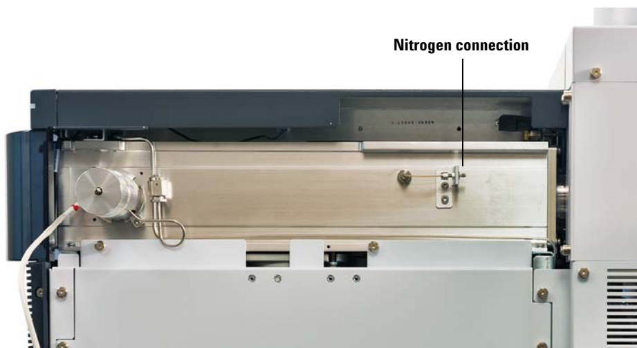
Figure 6 Collision cell nitrogen gas connection
