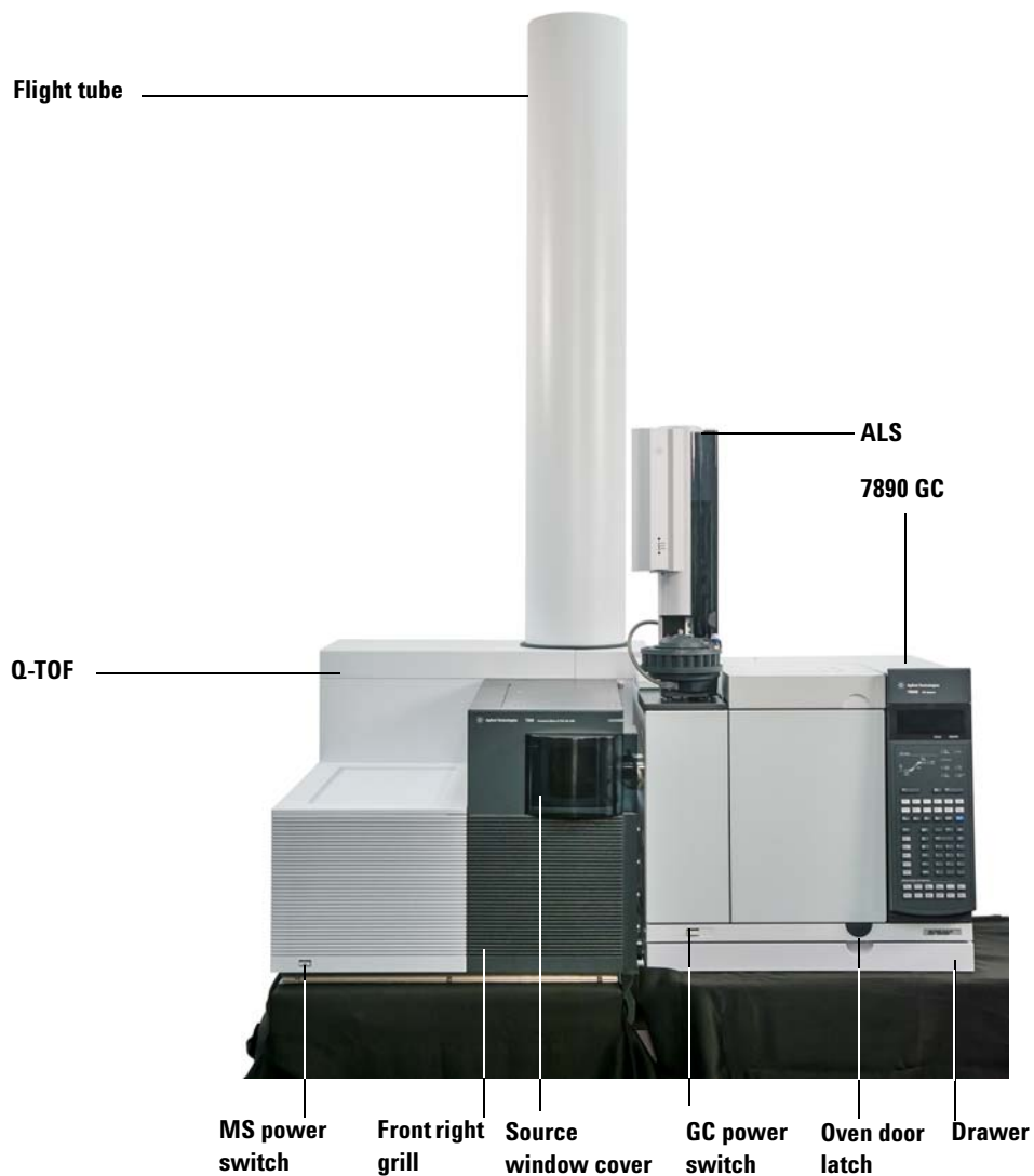
Figure 1 7250 Accurate-Mass Q-TOF GC/MS System
