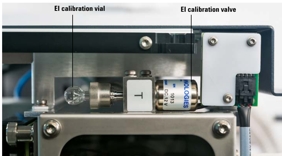
Figure 17 El calibration valve
