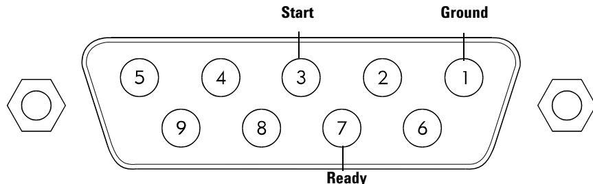
Figure 4 Remote start connector
